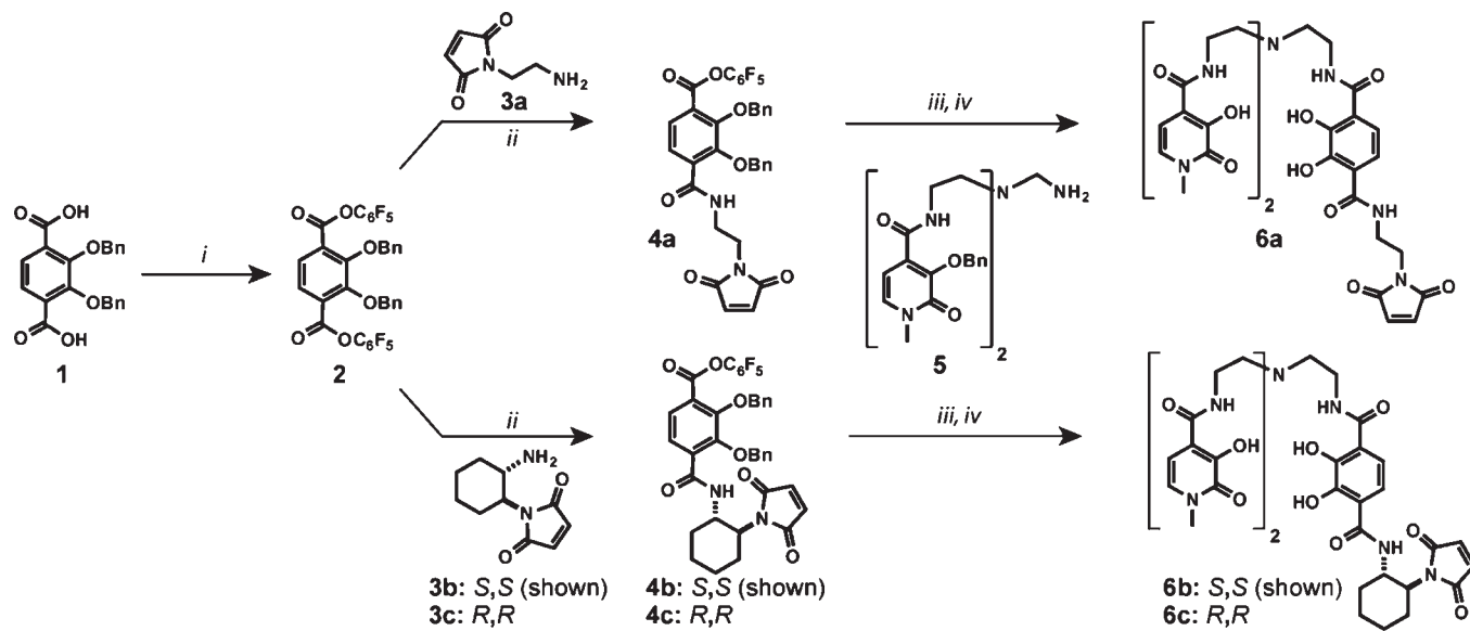
Scheme 1. Synthesis of Cysteine Reactive HOPO-Based Contrast Agents a
