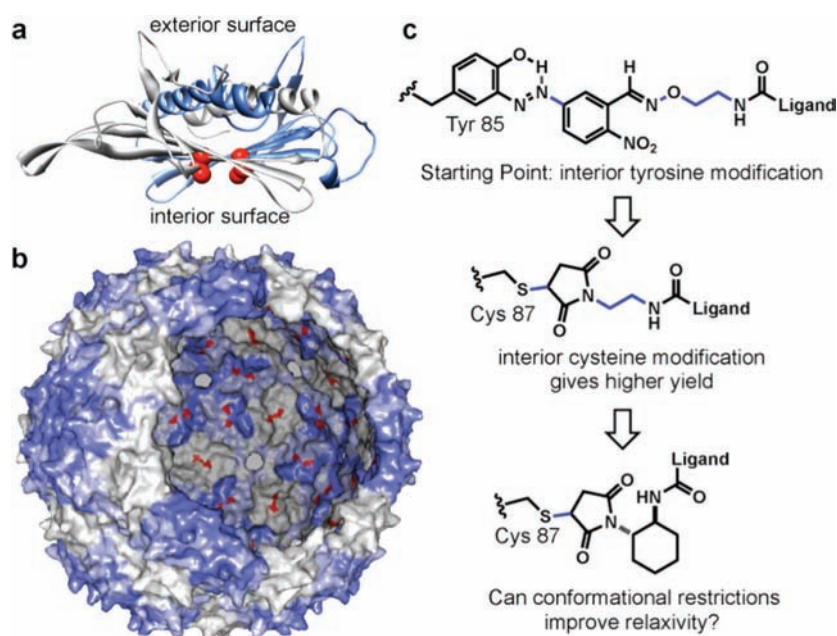
Figure 1. Design of highly efficient MRI contrast enhancement agents. (a) A crystal structure rendering of an MS2 coat protein dimer indicates the positions of the introduced cysteine residues (Cys 87) in red. (b) A rendering of the full 27 nm MS2 capsid shows the interior and exterior surfaces, with the 180 internal N87C positions highlighted in red. (c) The plan for increasing the overall relaxivity involved the use of more efficient cysteine modification chemistry and the rigidification of several rotatable bonds (indicated in blue).
