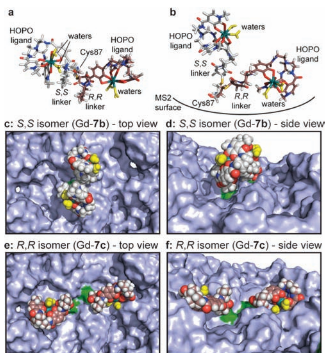
Figure 3. Models of sterically hindered Gd-HOPO complexes attached to the interior MS2 surface. Structures attached to two adjacent Cys87 groups were minimized simultaneously using MacroModel, and three different coordination isomers were considered for each. The Gd coordination spheres were based on a previously reported crystal structure. 43 Representative structures are shown here, with the full set appearing in Supporting Information Figures S5 through S8. Overlays of S,S (Gd-7b, gray) and R,R (Gd-7c, brown) complexes are shown for (a) a top view and (b) a side view. The rigid linker of S,S-complex Gd-7b (c and e) forces an upright conformation that leaves the water molecules (yellow) unobstructed. R,R-complex Gd-7c (d and f) places the water molecules much closer to the capsid surface, likely restricting their exchange. The Cys 87 attachment points are shown in green in c-f.
